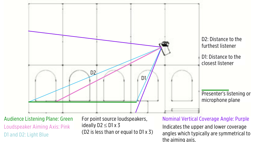
Figure 1. Determine the vertical horn pattern
